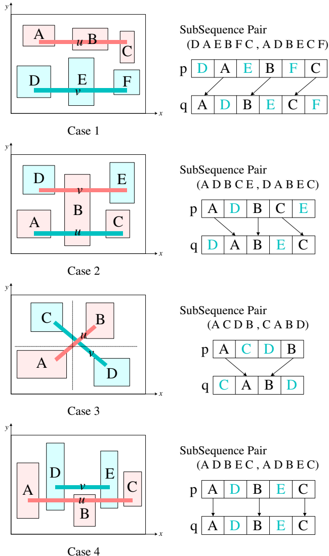
Figure 4: Cases of relative positions of two horizontal buses.
