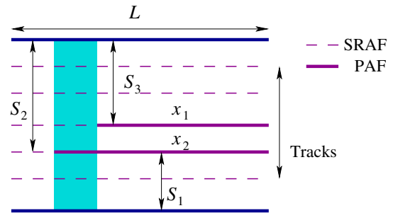
Fig. 5. Dummy metals are inserted for uniformity in a free region. Solid lines are PAF, and dashed lines are SRAF. One dashed line corresponds to a set of SRAF dummy metals, which are thin parallel wires. This region has 5 tracks. Its length is L .
