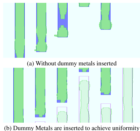
Fig. 1. Simulation results from Calibre. Without dummy metals inserted, the wires cannot be printed correctly even after OPC in (a). With dummy metals inserted, there are very little errors in (b). Defocus is considered in the aerial image simulation.
