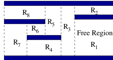
Fig. 4. Layout is partitioned into free regions. Dummy metals can be inserted for different free regions independently.
