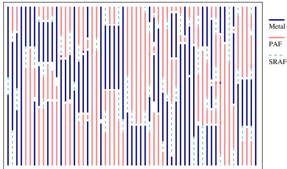
Fig. 8. Results from the dummy metal insertion algorithm. Dark lines are routed metal wires. Light lines are PAF. Dotted lines are SRAF.
