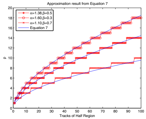
Fig. 7. p slowly increases with m . Equation 7 is a good approximation to the minimum p that satisfies Equation 6.
