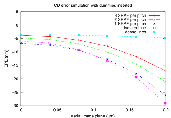
Fig. 2. Simulation results of DOF. The dense lines have the smallest EPE across all defocus levels and hence the best DOF. A larger EPE indicates a larger critical dimension (CD) error.
