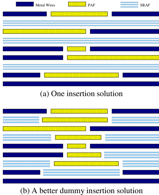
Fig. 3. Examples for coupling-aware SRAF/PAF dummy insertion. Solution in (b) is preferred with smaller coupling and lower lithography cost than the one in (a).
