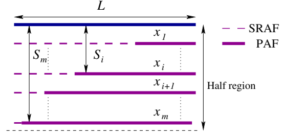
Fig. 6. Top half of free region with m tracks. It is symmetric to the bottom half.
