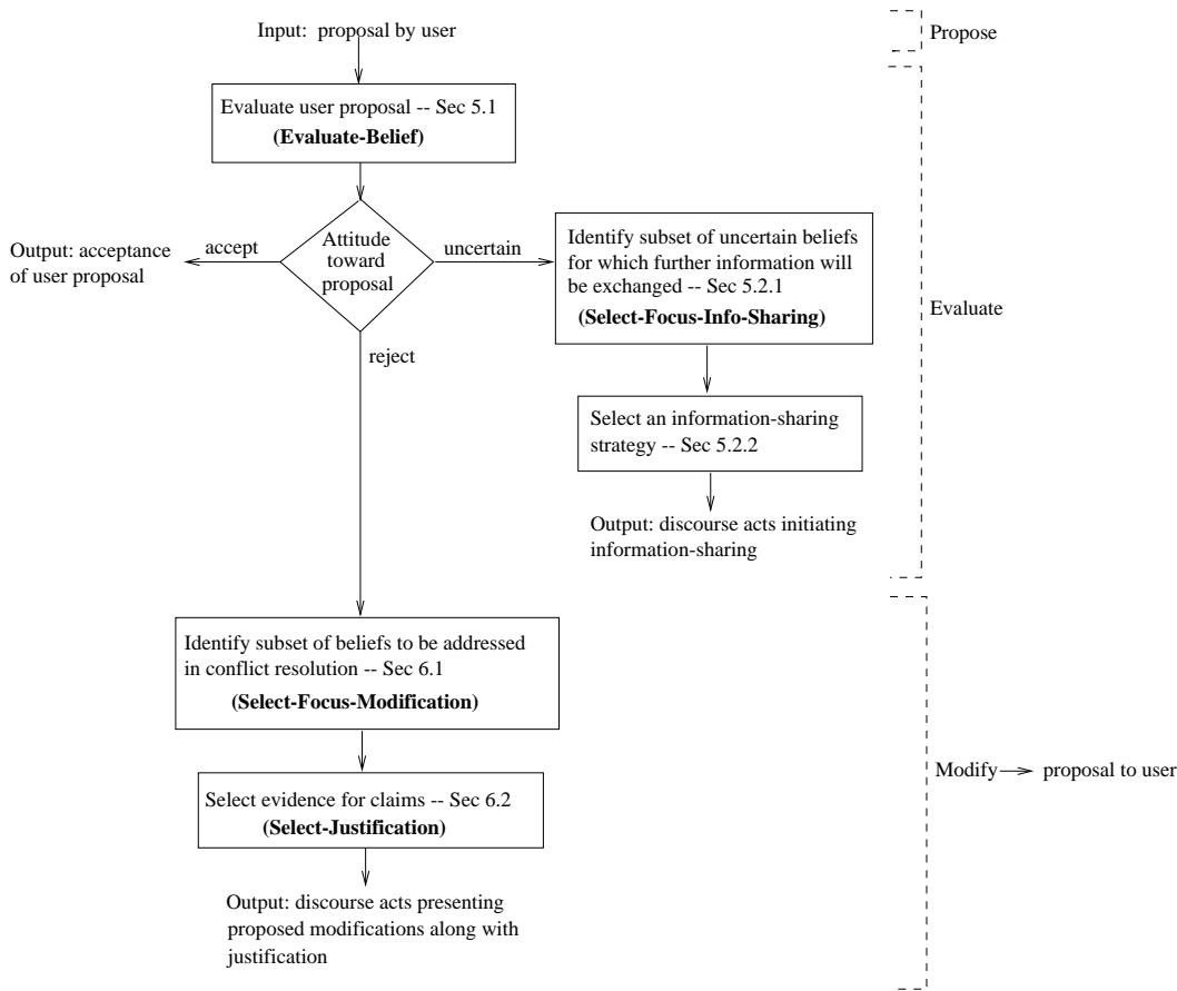
Figure 1 Schematic Diagram of Propose-Evaluate-Modify Process
