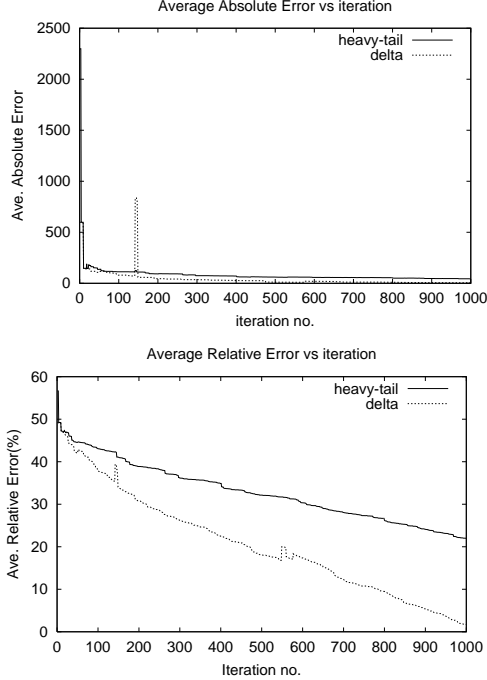
Figure 10: Convergence (fixed k ) . The estimation error averaged over an entire workload at each iteration of the learning process. This experiment shows how the estimation error is reduced as our XPathLearner learns the path selectivities from query feedback
