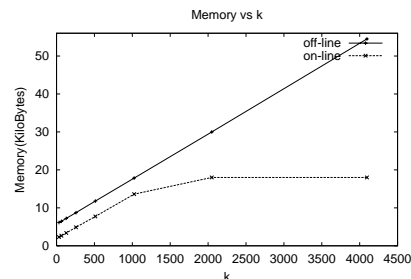
Figure 12: Memory vs k .
