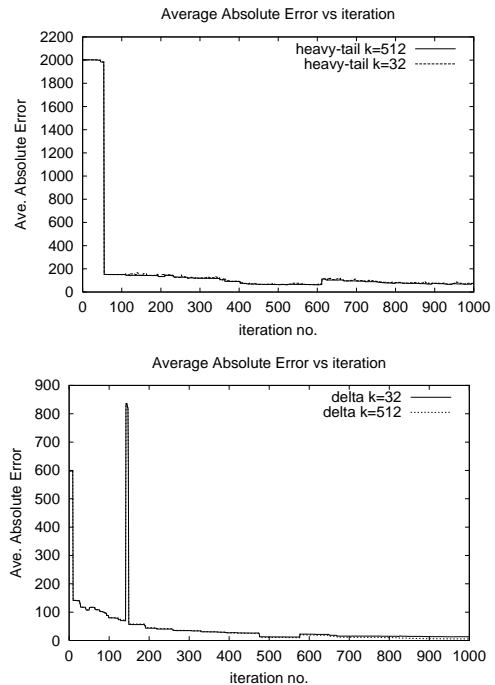
Figure 11: Convergence vs k . Estimation error averaged over an entire workload at each iteration of the learning process for two different values of k . The plot at the top is for the heavy-tail rule and the bottom one is for the delta rule. When k = 512 , all the tag-value counts are stored exactly. When k = 32 , only 32 tag-value counts are stored exactly.
