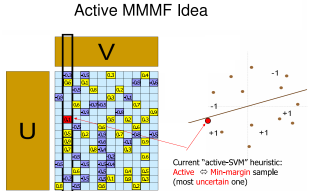
Fig. 1. Main idea of active learning in MMMF: choose the most “uncertain” sample next, where the distance to linear classifier (which we will also call “margin” here) measures the confidence in the prediction (i.e. we are least confident in predictions made for the instances closest to separating line between positive and negative examples). Note that the matrix is real-valued, with X_{ij} =distance (with sign) between feature-vector i and linear classifier j .
