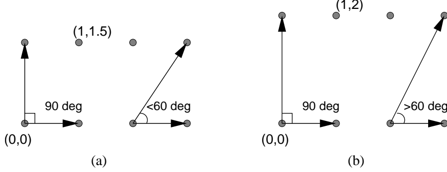
Figure 1: (a) The vectors comprising the lattice are denoted by circles. One of the lattice bases comprises two orthogonal vectors of lengths 1 and 1.5. Since 1.5 < \eta\left(\frac{\pi}{2}\right) = \sqrt{3} , the lattice possesses no other basis such that the angle between its vectors is at least \frac{\pi}{3} radians. (b) This lattice contains at least two \frac{\pi}{3} -orthogonal bases. One of the lattice bases comprises two orthogonal vectors of lengths 1 and 2. Here 2 > \eta\left(\frac{\pi}{2}\right) , and this basis is not the only \frac{\pi}{3} -orthogonal basis.
