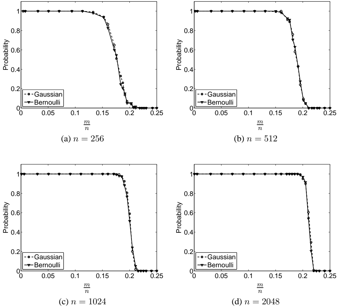
Figure 2: Empirical probability that a n \times m Gaussian or Bernoulli random matrix is \frac{\pi}{3} -orthogonal. At n = 256, 512, 1024, and 2048 and at m indicated by circles (for Gaussian) and triangles (for Bernoulli), we tested 200 randomly generated matrices. The empirical probability is the fraction of random matrices that were \frac{\pi}{3} -orthogonal.
