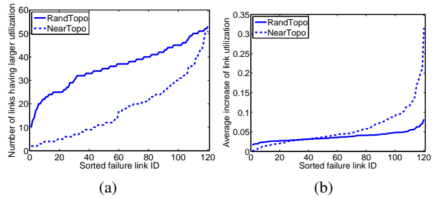
Figure 4: Link loads after failure under robust optimization. (a) Number of links experiencing load increase. (b) Average increase in link load.
