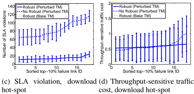
Figure 9: Impact of traffic uncertainty: hot-spot scenario. (a) and (b): Upload. (c) and (d): Download.
