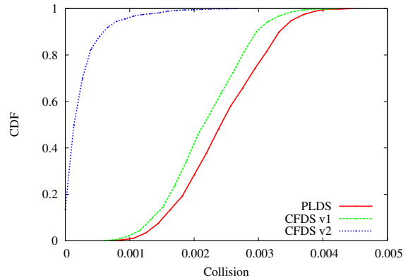
Figure 2. CDF for the ratio of collisions for active link-channel pairs.
