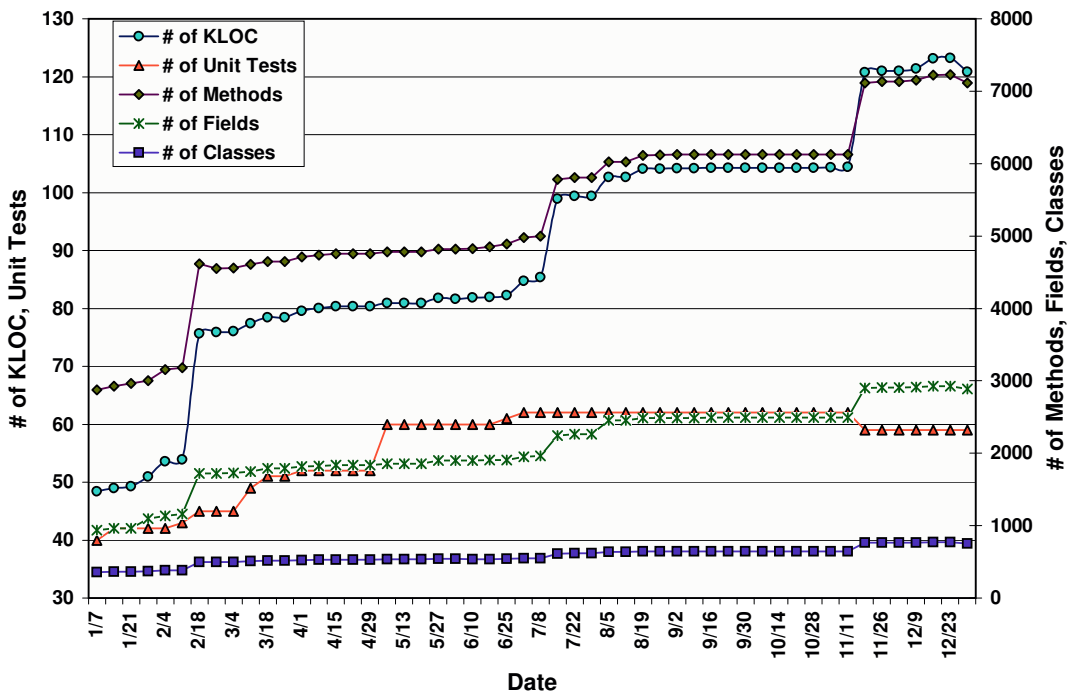
Figure 7: Daikon growth statistics for the year 2002
