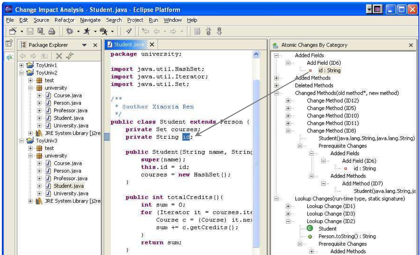
Figure 6: Snapshot of Chianti's atomic-changes-by-category view. The arrow shows how clicking on an atomic change opens an editor on the associated source fragment.
