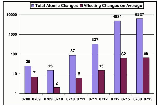
(b) Number of atomic changes and on average affecting changes on large interval and smaller daily intervals (note log scale)
