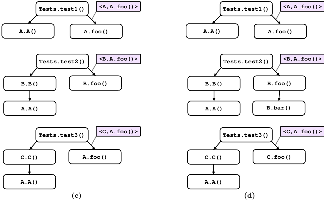
Figure 1: (a) Example program with 3 tests. Added code fragments are shown in boxes. (b) Atomic changes for the example program, with their interdependences. (c) Call graphs for the tests before the changes were applied. (d) Call graphs for the tests after the changes were applied.
