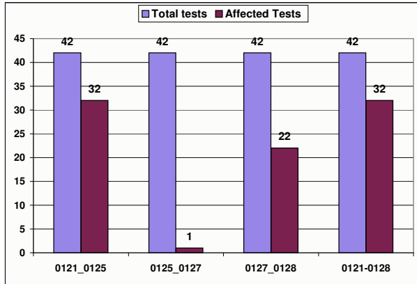
(a) Number of affected tests on large and smaller daily intervals.
