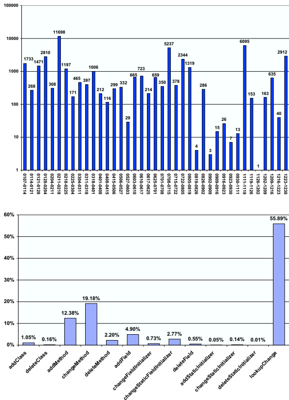
Figure 8: (a) Number of atomic changes between each pair of Daikon versions in 2002 (note the log scale). (b) Categorization of the atomic changes, aggregated over all Daikon edits in 2002.
