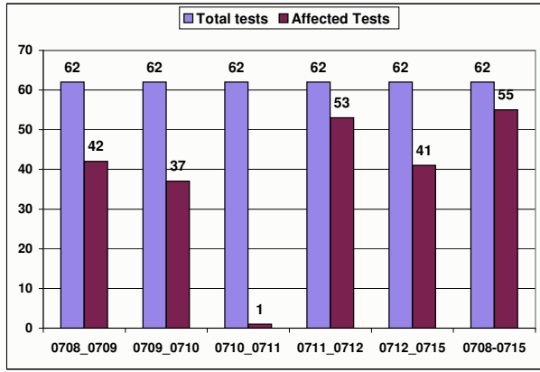
(a) Number of affected tests on large and smaller daily intervals.
