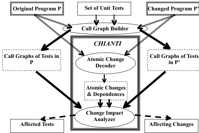
Figure 5: Chianti architecture.
